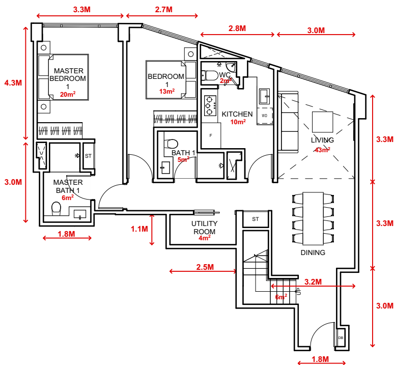
LOWER PENTHOUSE
