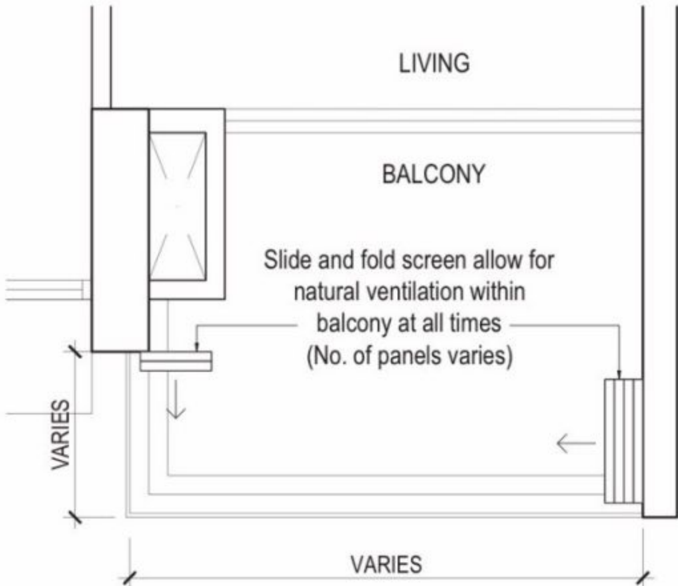
TYPICAL BALCONY PLAN
